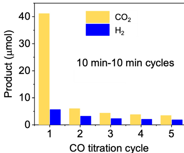
Fig. 6 Amount of \text{CO}_2 and \text{H}_2 produced during CO titration experiments at 450 °C. A schematic of the CO titration experiment and respective reactor outlet profiles are shown in Fig. S6†.
