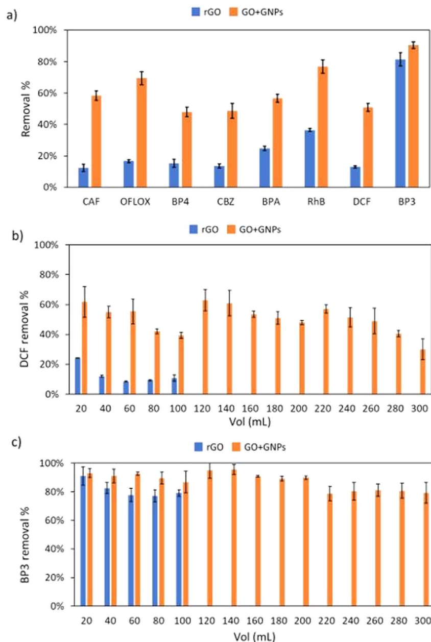
Fig. 7 (a) Average removal of a mixture of eight ECs (0.5 mg L -1 each in tap water, V tot = 100 mL, flow rate = 2.5 mL min -1 ) by aerogels of rGO (blue) and GO + GNPs (orange); removal of (b) diclofenac (DCF) and (c) benzophenone-3 (BP3) (0.5 mg L -1 each in tap water, V tot = 300 mL, flow rate = 2.5 mL min -1 ).
