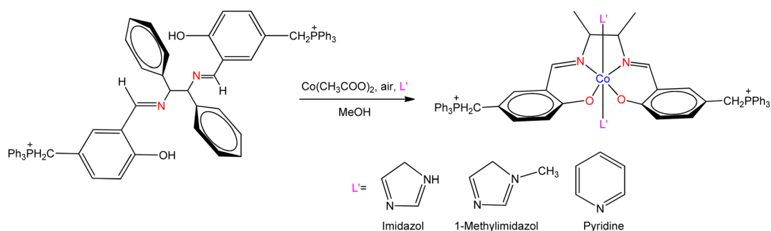
Fig. 14 Schematic representation of SB and its \text{Co(III)} complexes containing phosphonium ion.
