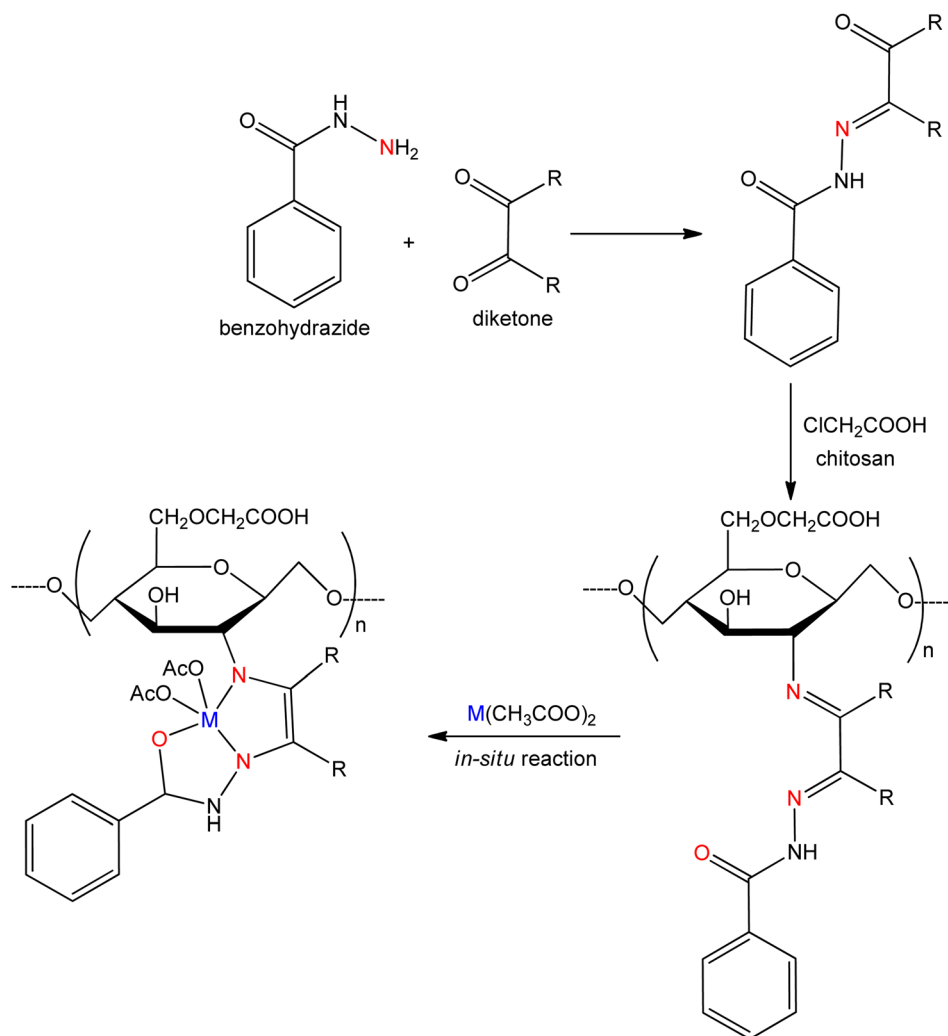
Fig. 13 Synthesis of water-soluble hydrazide based O -carboxymethyl chitosan SB and its metal complexes ( M = \text{Cu}, \text{Zn} ).
