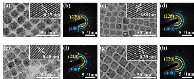
Fig. 2 TEM and HRTEM images (insets) of (a) \text{Cs}_2\text{AgInCl}_6 , (c) 2%B, (e) 20%Yb, 7%Er and (g) 2%B@20%Yb, 7%Er NCs, and their corresponding SAED patterns (b), (d), (f) and (h). Some 'dark dots' appearing in the TEM images over the surface of the NCs are attributable to the reduction of \text{Ag}^+ to \text{Ag}^0 by Olam. 21,34
