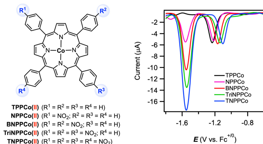
Fig. 12 Cobalt(III) tetraphenylporphyrin complexes and their differential pulse voltammograms in DMF with 0.1 M [t n Bu 4 N][PF 6 ]. Reproduced from ref. 66 under a Creative Commons License CC-BY-NC-ND 4.0.
