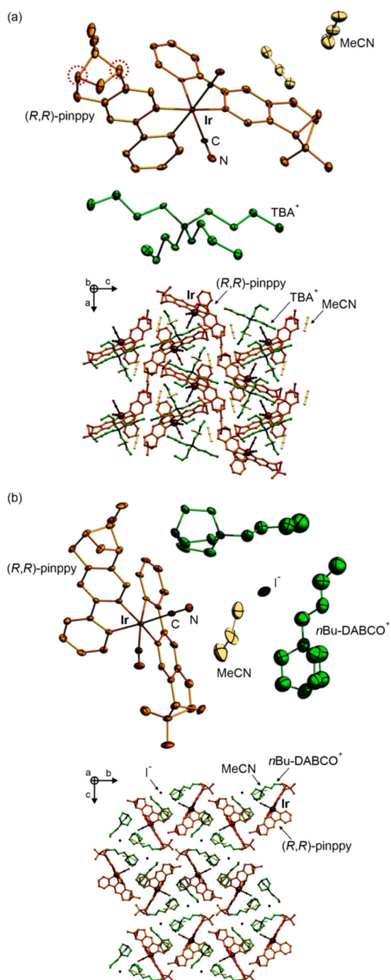
Fig. 1 The representative views on the crystal structures of 1 (a) and 2 (b), including the molecular building units (top parts) and the supra-molecular arrangements of molecular components (bottom parts). The chiral ligand, heavy atoms, cyanido ligands, solvent molecules, and counter-ions are labeled. The atoms in the top parts were presented as thermal ellipsoids at the 40% and 35% probability levels for 1 and 2 , respectively.
