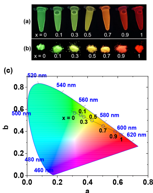
Fig. 5 Images of (a) aqueous solution samples and (b) powder samples of \text{GdEu}_x\text{Tb}_{1-x}\text{O}_3@(\text{PAA}/\text{PDA}) nanoparticles ( x = 0, 0.1, 0.3, 0.5, 0.7, 0.9 , and 1 ) under 254\text{ nm} UV irradiation, illustrating the colour tuning between green and red by adjusting x . (c) CIE (1931) chromaticity system, showing the colour tuning between green and red.
