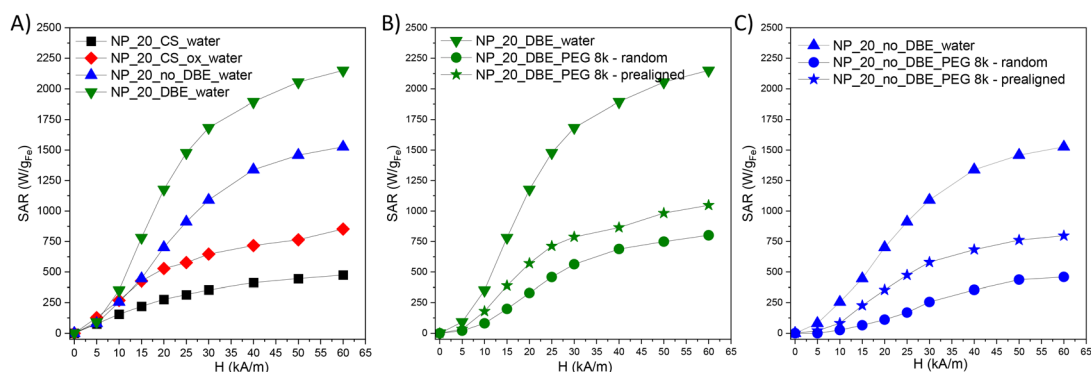
Fig. 5 (A) SAR values for NP_P20_DBE, NP_P20_no_DBE, NP_20_CS and NP_20_CS_ox suspensions in water and of (B) NP_20_DBE and (C) NP_20_no_DBE suspended in water and in a PEG8k matrix, random or prealigned, at a concentration of 1 \text{ mg}_{\text{Fe}} \text{ mL}^{-1} .
