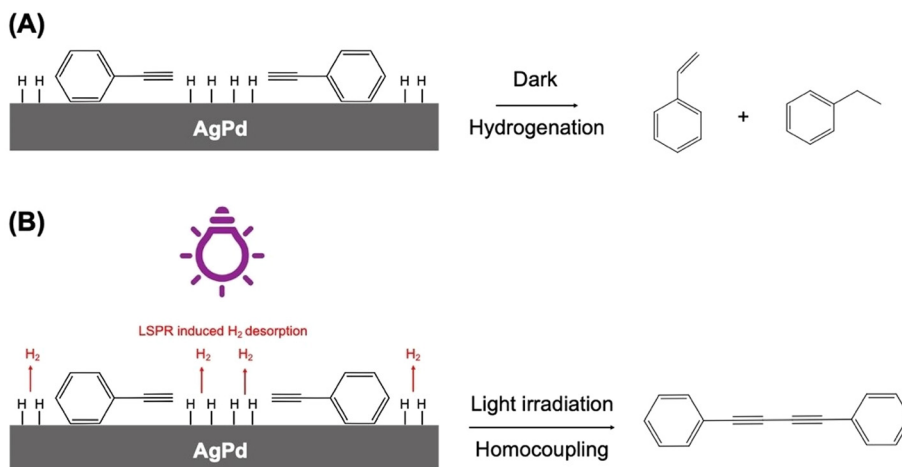
Fig. 18 Proposed mechanisms for phenylacetylene conversion by AgPd/ZrO 2 NPs. (A) Under dark conditions, conversion follows the hydrogenation pathway in which adsorbed H 2 species are added to surface species, leading to the formation of styrene and ethylbenzene as the main products. (B) Under light irradiation, LSPR hot carriers drive H 2 desorption from the surface, depleting the concentration of H surface species. This changes the reaction pathway to homocoupling and leads to the formation of 1,4-diphenylbutadiyne as the main product. "Reproduced from ref. 108 with permission from John Wiley and Sons, copyright 2023".
