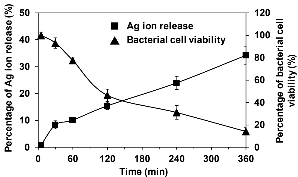
Figure 7. Correlation with silver ion release rate and bacterial cell viability
