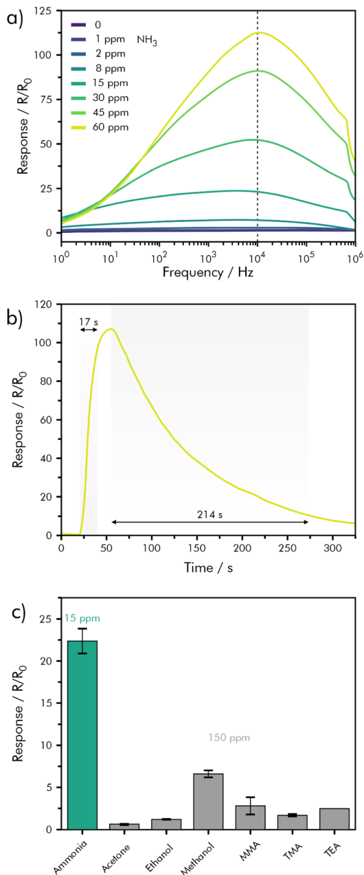
Fig. 12 Hybrid NFI-rGO sensing performance (a) relative response variation as a function of frequency for NH_3 concentrations from 0–60 ppm; (b) dynamic response–recovery curve for exposure to 60 ppm of NH_3 ; (c) cross-sensitivity between NH_3 (15 ppm), acetone, ethanol, methanol, monomethylamine (MMA), trimethylamine (TMA) and triethylamine (TEA) (150 ppm); redrawn and adapted, with permission from ref. 146.
