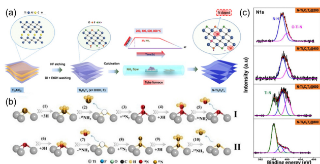
Fig. 5 (a) Illustration of synthesis of N-doped MXene from the \text{Ti}_3\text{AlC}_2 MAX phase. 62 Copyright 2019, American Chemical Society. (b) The proposed N dopants in 15N doped-TiV- \text{Ti}_{3-x}\text{C}_2\text{T}_y-1.2 MXene catalysts act as an active catalytic site in ENRR. 63 Copyright 2021, Elsevier. (c) Core-level XPS of the N 1s of N-doped MXene samples annealed at various temperatures. 63 Copyright 2021, Elsevier.
