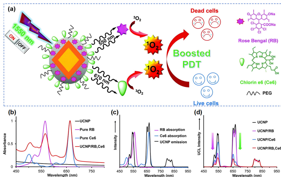
Fig. 8 (a) Schematic diagram of the formation of \text{UCNP}@/\text{SiO}_2/\text{RB,Ce6} . (b) The absorbance of UCNPs, RB, Ce6, UCNPs/RB,Ce6. (c) The absorption and emission spectra of RB, Ce6 and UCNPs respectively. (d) The UCL spectra of UCNPs, UCNPs/RB, UCNPs/Ce6 and UCNPs/RB,Ce6 under irradiation at 1550 nm. Reproduced with permission from ref. 58. Copyright 2014, The Royal Society of Chemistry.
