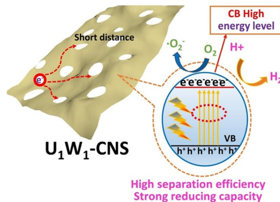
Fig. 10 Schematic illustration of porous GCN. Reprinted with permission from ref. 74 Copyright 2021, Elsevier.
