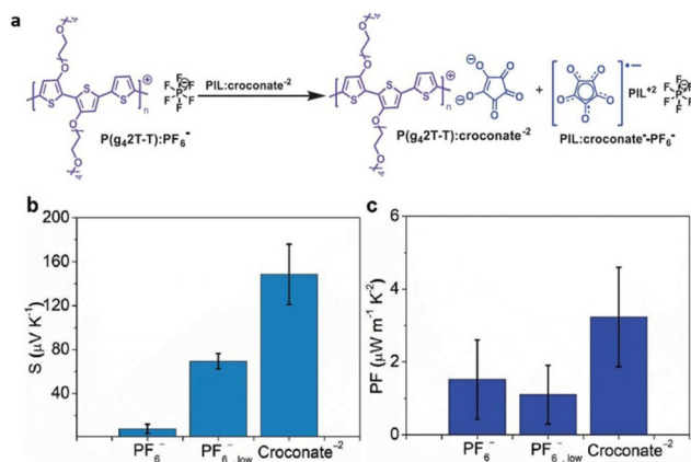
Fig. 54 (a) Structure of the P(g42T-T) with croconate 2- . Thermoelectric parameters of chemically doped and ion exchange P(g42T-T) films. (b) Seebeck coefficients ( S ) and (c) power factors ( PF ) of P(g42T-T): \text{PF}_6^- , P(g42T-T): \text{PF}_6^-_{\text{low}} , and P(g42T-T): croconate 2- thin films. Reproduced from ref. 234 with permission from Wiley-VCH, Copyright [2023].
