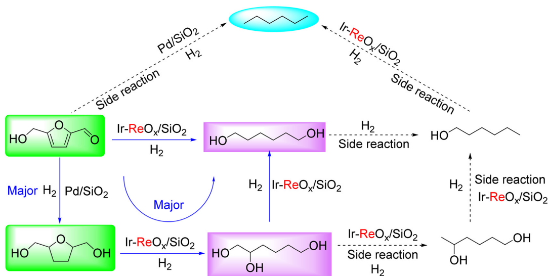
Fig. 21 Reaction routes of hydroxymethylfurfural conversion to 1,6-hydrodeoxylation over Pd/SiO 2 + Ir-ReO x /SiO 2 catalysts. 182
