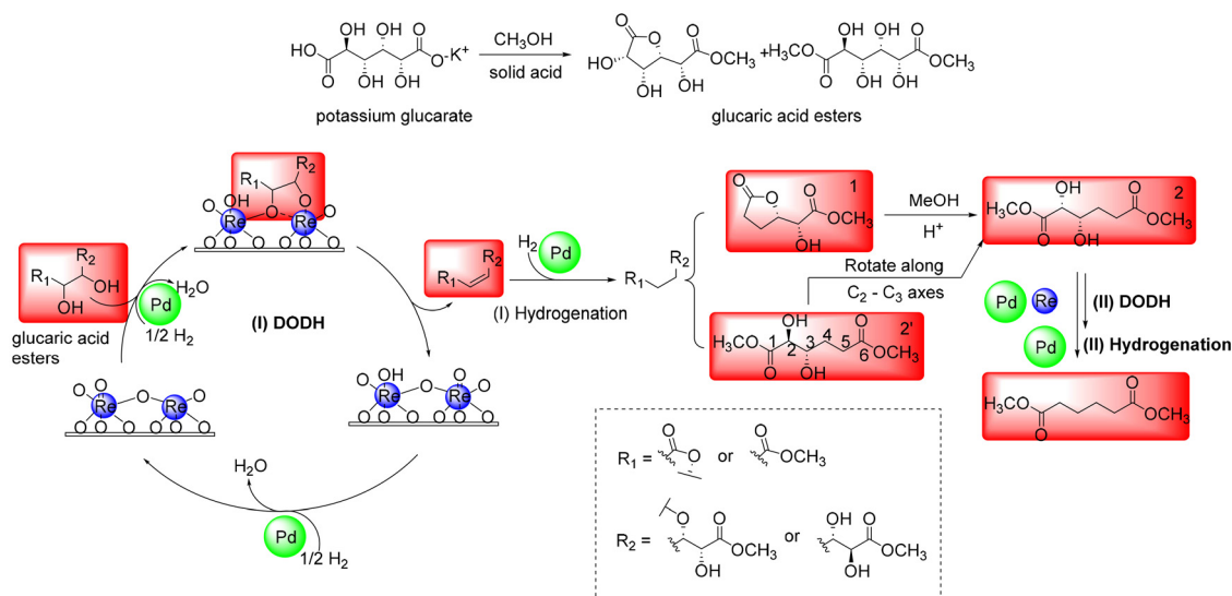
Fig. 19 Proposed reaction mechanism for the conversion of glucaric acid (potassium glucarate) to adipic acid (methyl adipate) catalyzed by Pd-ReO x /AC 175 (DODH: deoxydehydrogenation).
