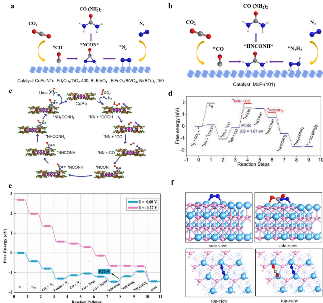
Fig. 11 (a) \text{CO} and \text{N}_2 intermediates pathway for urea synthesis. (b) \text{CO} and \text{N}_2\text{H}_2 intermediates pathway for urea synthesis. (c) \text{N}_2 and \text{CO}_2 co-reduction steps for urea synthesis on CuPc. (d) The full free energy profile of urea synthesis and hydrogen adsorption on Cu center. Reproduced from ref. 143, with permission from Wiley-VCH, copyright 2022. (e) The computed free energy profiles for urea electrocatalytic on Mo-terminated MoP-(101) surface at applied potentials. (f) The optimized geometrical structures for \text{N}_2 and \text{N}_2 + \text{CO}_2 adsorption on MoP-(101) surface. Reproduced from ref. 109, with permission from Royal Society of Chemistry, copyright 2023.
