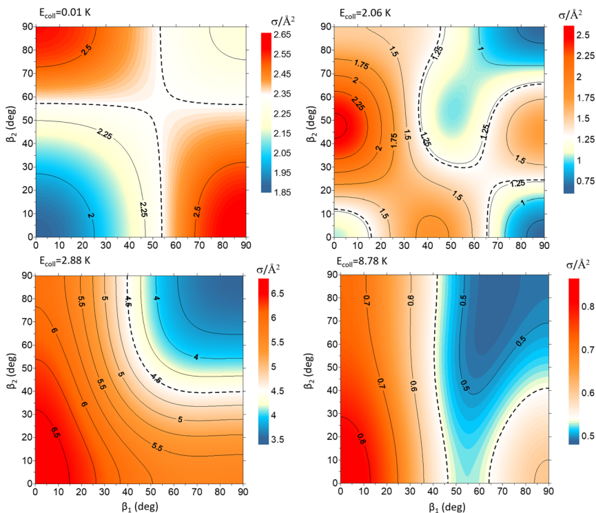
Fig. 3 Contour maps showing the ICS \sigma^{\beta_1\beta_2} for D_2(\nu=0, j=2) + D_2(\nu=2, j=2) \rightarrow D_2(\nu=0, j=2) + D_2(\nu=2, j=0) collisions as a function of \beta_1 and \beta_2 for each of the four values of E_{\text{coll}} indicated in Fig. 1. \beta_1 is the angle that defines the direction of the internuclear axis of the D_2(\nu=0, j=2) , whose internal state does not change in the collision, whereas \beta_2 refers to the D_2(\nu=2, j=2) molecule that experiences the quenching of its rotational level.
