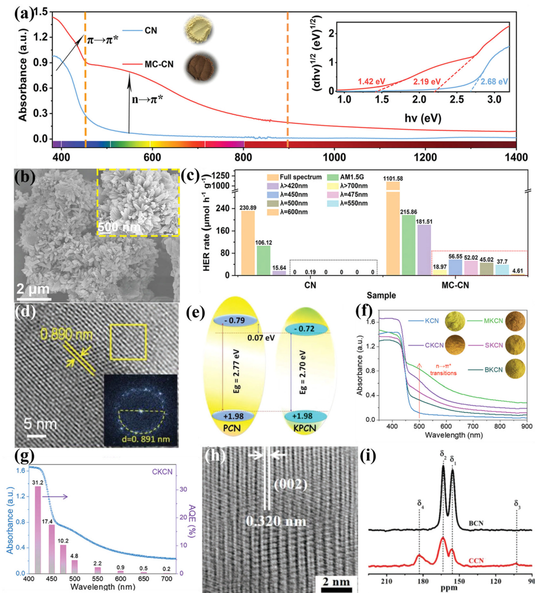
Fig. 11 (a) UV-vis diffuse reflectance spectra (DRS) of CN and MC-CN and the corresponding Kodelka–Munk plots (inset). (b) SEM and high magnification SEM images (inset) of MC-CN. (c) Wavelength dependence of the photocatalytic \text{H}_2 generation rate of CN and MC-CN. Reproduced with permission. 129 Copyright 2022, Wiley-VCH. (d) HRTEM image and FFT pattern (inset) of KPCN. Reproduced with permission. 95 Copyright 2019, Wiley-VCH. (e) Schematic representation of the band structures of PCN and KPCN. Reproduced with permission. 95 Copyright 2019, Wiley-VCH. (f) UV-vis-NIR DRS spectra of KCN, MKCN, CKCN, SKCN, and BKCN samples. (g) Wavelength dependence of AQE of CKCN. Reproduced with permission. 131 Copyright 2022, Wiley-VCH. (h) HRTEM image of CCN. (i) ^{13}\text{C} NMR of BCN and CCN. Reproduced with permission. 88 Copyright 2019, Wiley-VCH.
