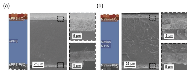
Fig. 3 Cross-sections of (a) sulfonated poly(phenylene sulfone) (sPPS)-MEA and (b) Nafion-MEA by spray coating. Reproduced with permission from ref. 127. Copyright 2020, WILEY-VCH.
