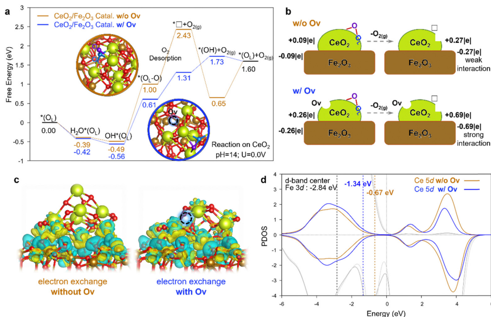
Fig. 6 DFT calculations for LOM-based OER catalyzed by the \text{Fe}_2\text{O}_3@/\text{CeO}_2\text{-O}_v and \text{Fe}_2\text{O}_3@/\text{CeO}_2 catalysts. (a) Free energy diagram for LOM-based OER steps. The detailed 3D configurations are shown in Fig. S40 (ESI ^\dagger ). Color code: Ce in yellow; Fe in brown; the O about to be removed in LOM in blue; the O from water in purple; the other O in red. The dotted lines represent the \text{O}_2 desorption step. (b) Illustration of Bader charge changes during the \text{O}_2 desorption step. (c) Charge density diagram showing the electron exchange between the \text{CeO}_2 cluster and \text{Fe}_2\text{O}_3 support of the ^*\square intermediate after \text{O}_2 desorption. Electron depletion and accumulation are depicted by yellow and blue areas, respectively. The isosurfaces are plotted at the value of \pm 0.03 |e| \text{\AA}^{-3} . (d) Projected density of states (PDOS) of Ce 5d orbitals in the ^*\square intermediate of \text{CeO}_2/\text{Fe}_2\text{O}_3 catalysts. The lighter and darker gray lines show the PDOS of surface Fe atoms with and without \text{O}_v on \text{CeO}_2 , respectively. The yellow and blue numbers show the d-band-center of Ce without and with \text{O}_v .
