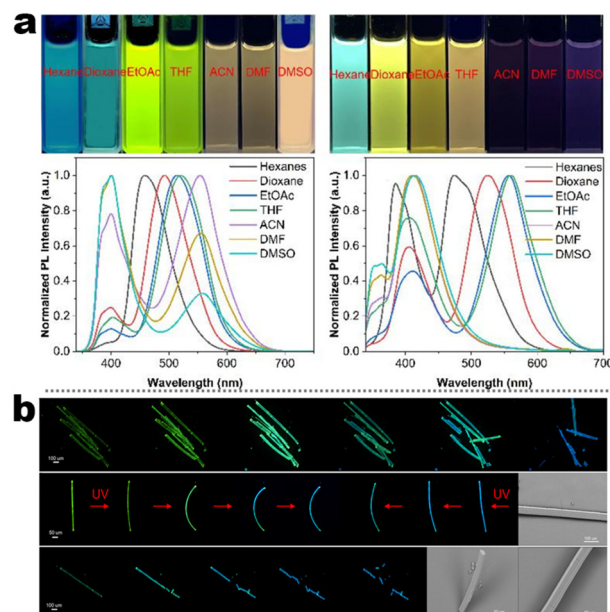
Fig. 15 (a) Fluorescence color changes under 365 nm UV light and fluorescence spectra of 4-14 . Reproduced from ref. 100 with permission. Copyright (2023), Wiley Online Library. (b) Images of photosalience and photochromism of 4-15 crystals. Reproduced from ref. 108 with permission. Copyright (2023), The Royal Society of Chemistry.
