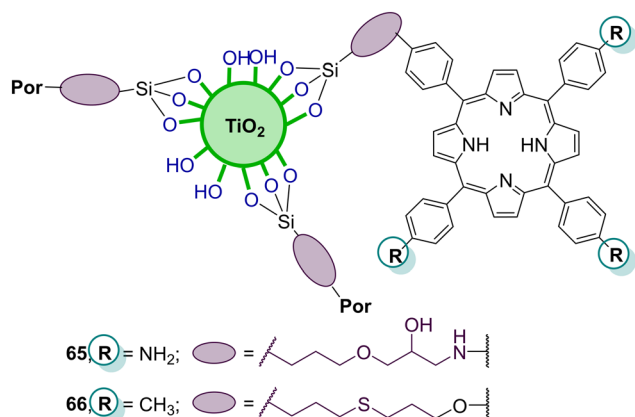
Fig. 21 Representation of \text{H}_2\text{65-TiO}_2 and \text{H}_2\text{66-TiO}_2 .
