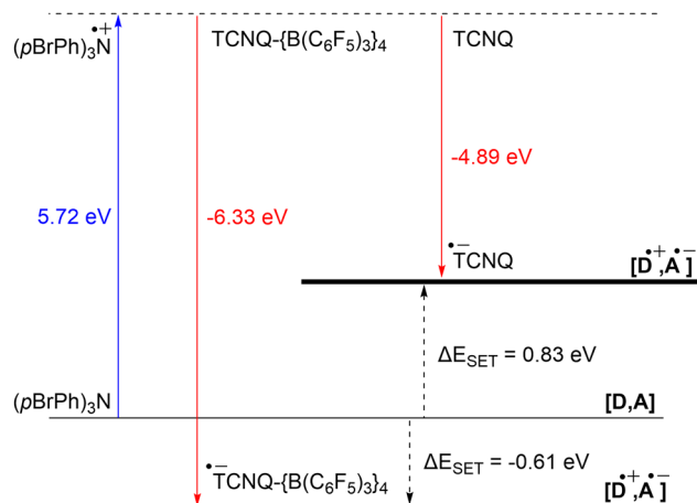
Fig. 12 Energy diagram with calculated ionisation energy (IE) of (p\text{BrPh})_3\text{N} (blue) and electron affinities (EA) of TCNQ and \text{TCNQ}\{-\text{B}(\text{C}_6\text{F}_5)_3\}_4 (both red) for DCM. For both electron acceptors are the \Delta E_{\text{SET,calc}} indicated (black arrows).
