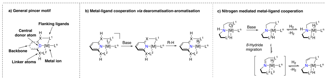
Scheme 2 (a) General pincer complex structure; (b) base induced dearomatisation–aromatization MLC activation mode of Milstein pyridyl type pincer complexes; (c) base induced MLC activation modes of NH-only type pincer complexes.
