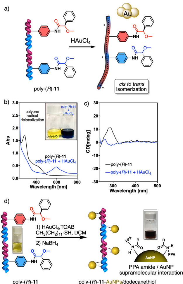
Fig. 48 (a) Schematic representation for the formation of radicals in poly-(R)-11 in presence of \text{HAuCl}_4 . (b) UV-vis and (c) CD spectra of poly-(R)-11 and poly-(R)-11 in presence of \text{HAuCl}_4 . (d) Schematic representation for the formation of poly-(R)-11-AuNPs nanocomposites by a variation of Brust-Schiffrin method. Reproduced from ref. 247 with permission from John Wiley and Sons, copyright 2021.
