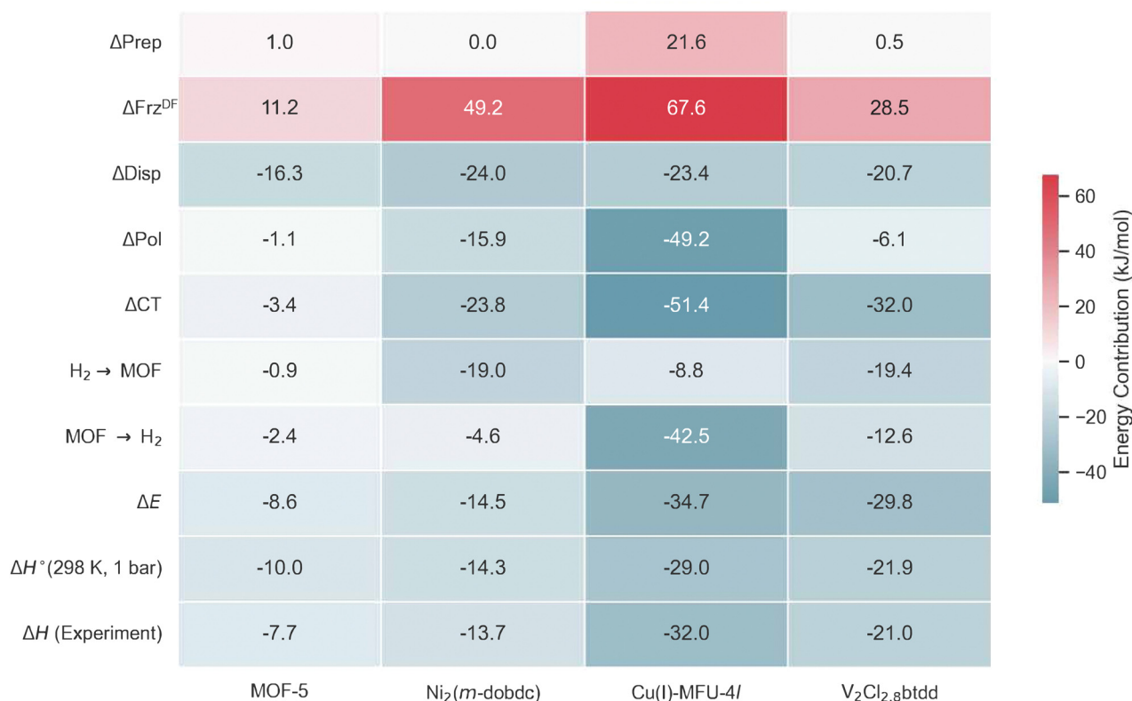
Fig. 9 A comparative summary of energy decomposition analysis (EDA) (see eqn (2) for definition of terms) of H 2 binding to four MOFs. \Delta\text{CT} contains forward (H 2 → MOF) and back-donation (MOF → H 2 ) contributions. The MOFs are MOF-5, a material with no open metal sites (see Fig. 5), the Lewis acidic Ni(II) site in Ni 2 ( m -dobdc) (see Fig. 6), and \pi -basic Cu(I) and V(II) sites in Cu(I)-MFU-4l (see Fig. 7) and V 2 Cl 2.8 (btdd) (see Fig. 8) respectively. \Delta H^\circ(T) values are reported at 298 K and 1 bar, and compared to experimental values.
