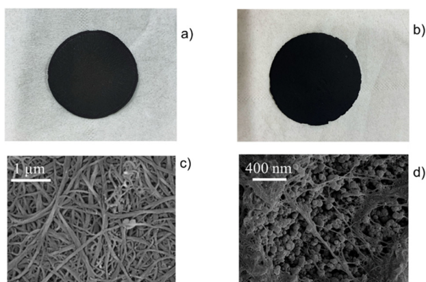
Fig. 13 Photographs of neat SWCNT-BP (a) and bioMOF@SWCNT-BP (b) obtained by integrating Cu 6 SrThreo and SWCNT-BP. The membranes own an average diameter of 41 \pm 1 mm. SEM images of SWCNT-BP (c) and bioMOF@SWCNT-BP (d). This figure is reproduced with permission from ref. 78, copyright ACS 2022.
