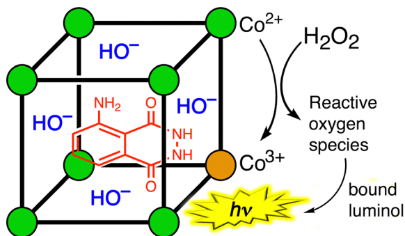
Fig. 12 Cartoon representation of the oxidation of luminol by \text{H}_2\text{O}_2 catalysed by the cage \text{H}^{\text{W}} which (i) binds the guest, (ii) uses its \text{Co(II)/Co(III)} redox couple to activate the \text{H}_2\text{O}_2 generating reactive oxygen species surrounding the cage surface, and (iii) tethers any hydroxide ions required for the reaction in place via the cage positive charge.
