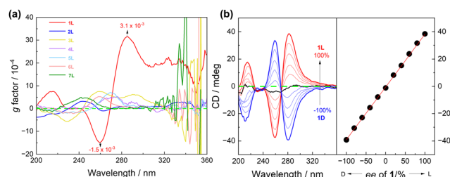
Fig. 4 (a) Wavelength profiles of the g factors of 1L – 7L in \text{CH}_3\text{CN} . [ 1L – 5L ] = 10 \mu\text{M} , [ 6L ] = 40 \mu\text{M} , and [ 7L ] = 20 \mu\text{M} . (b) CD spectra of mixtures of 1L and 1D of various ee in \text{CH}_3\text{CN} and plots of the CD signals at 281 nm against ee. [ 1L ] + [ 1D ] = 10 \mu\text{M} .
