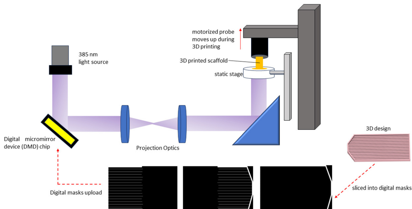
Fig. 1 Schematic of the DLP-based 3D printing system. Digital masks were sequentially uploaded to the synchronized, computerized 3D printing system. The DMD chip then adjusted their micromirror orientation according to the digital pattern uploaded into the synchronized 3D printing system. The 385 nm light projected from the light source was reflected off the DMD chip as patterned light and was projected through a series of projection lens to ultimately reach the focal plane within the static stage that contained the prepolymer reservoir. PGSA prepolymer was then photocrosslinked into a 3D-printed structure as the motorized probe moved up in a layer-by-layer fashion during the printing process.
