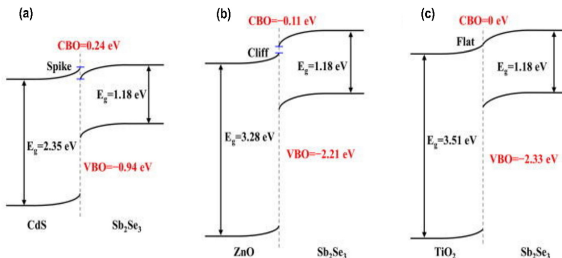
Fig. 7 Schematics of the band alignments between \text{Sb}_2\text{Se}_3 and different buffer layers (a) CdS, (b) ZnO, and (c) \text{TiO}_2 . 111
