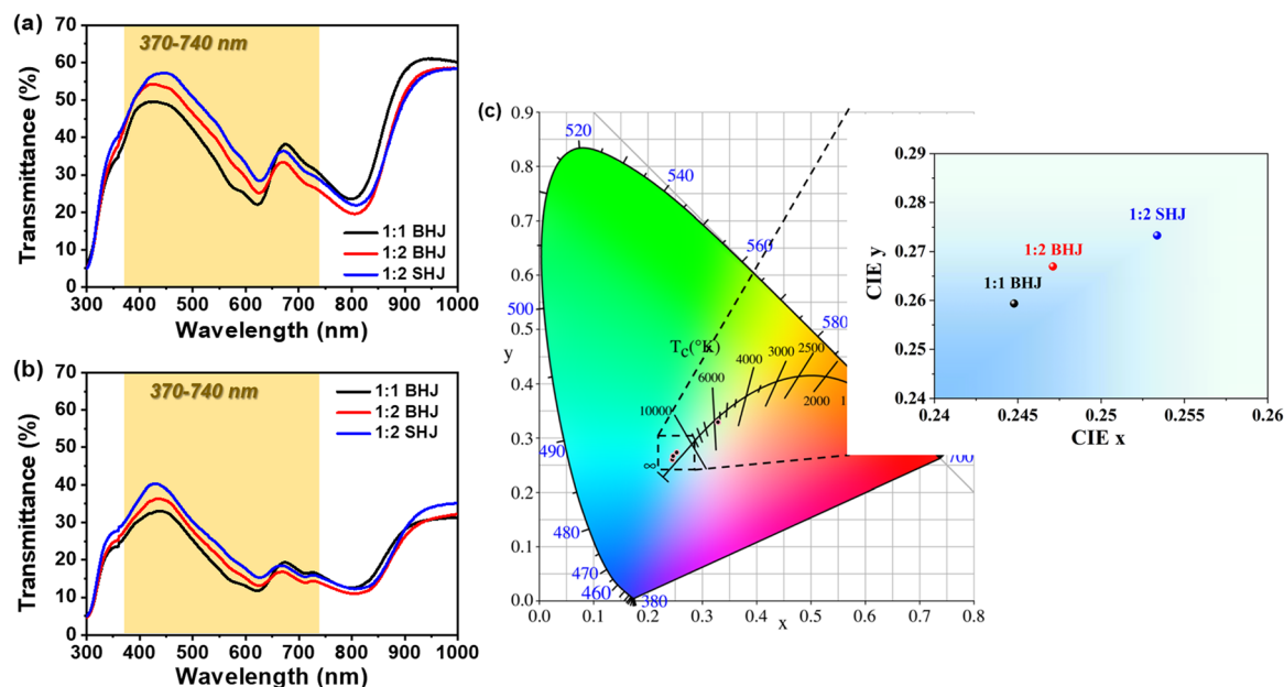
Fig. 3 Transmittance spectra of (a) blend films and (b) the corresponding ST-OSCs based on 1:1 BHJ, 1:2 BHJ and 1:2 SHJ. (c) Colour coordinates of the ST-OSCs on a CIE chromaticity diagram.
