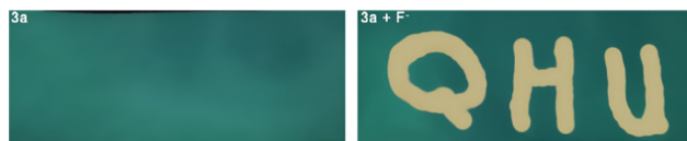
Fig. 5 The 3a based film sensors for fluoride anions under UV irradiation ( \lambda_{\text{ex}} = 365 nm).
