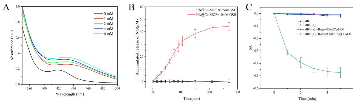
Fig. 4 (A) HN@Cu-MOF-mediated GSH consumption. (B) The accumulated release of NO from the HN@Cu-MOF with or without GSH. (C) The detection of \cdot\text{OH} release of the HN@Cu-MOF.
