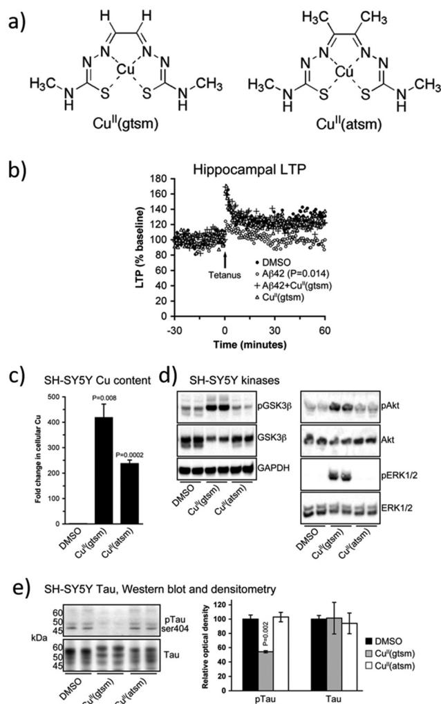
Fig. 5 (a) Structures of [Cu^{II}(gtms)] and the control [Cu^{II}(atms)] . (b) Whereas A\beta_{42} inhibits the hippocampal long-term potentiation (LTP) by 28%, this is prevented when treated with [Cu^{II}(gtms)] . (c) In vitro , [Cu^{II}(gtms)] increases the cellular levels of Cu. (d) Western blot analyses show that [Cu^{II}(gtms)] induces the phosphorylation of kinases GSK3 \beta , Akt, and ERK1/2. (e) [Cu^{II}(gtms)] inhibits tau phosphorylation at ser404 without affecting the abundance of total tau. Adapted from Ref. 68. Reproduced with permission.
