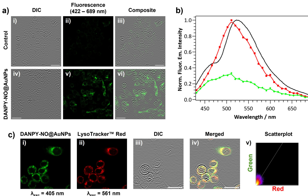
Fig. 3 (a) CLSM images of RAW264.7γ NO − cells untreated (i)–(iii) and incubated with DANPY-NO@AuNPs (4.2 μg mL −1 , overnight) (iv)–(vi); images collected using λ exc = 405 nm and Δλ em = 422–689 nm. Scale bars = 25 μm. (b) Normalised fluorescence emission spectrum of: DANPY-NO@AuNPs in DMEM cell culture medium recorded in the fluorescence spectrophotometer (black); RAW264.7γ NO − cells incubated with DANPY-NO@AuNPs recorded in the CLSM (red); and control cells without DANPY-NO@AuNPs loaded recorded in the CLSM (green); λ exc = 405 nm. (c) CLSM images of RAW264.7γ NO − cells incubated with DANPY-NO@AuNPs (4.2 μg mL −1 ) and LysoTracker™ Red DND-99 (5 μM) (i)–(iv) and scatterplot showing the correlation between the green and red emission intensities (v). Images collected upon excitation at (i) λ exc = 405 nm, Δλ em = 500–580 nm and (ii) λ exc = 561 nm, Δλ em = 580–625 nm; (iii) DIC channel; and (iv) composite image of green, red and DIC channels. Pearson's coefficient of 0.73 ± 0.04 ( n = 3 images, ca. 20 cells). Scale bars = 20 μm.
