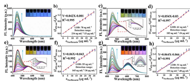
Fig. 4 (a) Plots of fluorescence emission spectra after the addition of NOR with different concentrations to COF BMTH-TFB ( \lambda_{\text{ex}} = 370\text{ nm} ) (the inset shows the fluorescence color change of the COF BMTH-TFB solution). (b) A linear plot between the NOR concentration and (I_{450\text{ nm}} - I_0)/I_0 . (c) Fluorescence emission spectra after the addition of NOR with different concentrations to COF BMTH-TB ( \lambda_{\text{ex}} = 370\text{ nm} ) (the inset shows the fluorescence color change of COF BMTH-TB solution). (d) Linear plot between NOR concentration and (I_{450\text{ nm}} - I_0)/I_{520\text{ nm}} . (e) Fluorescence emission spectra after the addition of NOR with different concentrations to COF BMTH-TBT ( \lambda_{\text{ex}} = 370\text{ nm} ) (the inset shows the fluorescence color change of the COF BMTH-TBT solution). (f) A linear plot between the NOR concentration and (I_{450\text{ nm}} - I_0)/I_{564\text{ nm}} . (g) Fluorescence emission spectra after the addition of NOR with different concentrations to COF BMTH-HB ( \lambda_{\text{ex}} = 370\text{ nm} ) (the inset shows the fluorescence color change of the COF BMTH-HB solution). (h) The linear plot between the NOR concentration and (I_{450\text{ nm}} - I_0)/I_{613\text{ nm}} .
