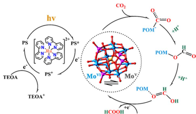
Scheme 7 Proposed mechanism for the photocatalytic \text{CO}_2 reduction to \text{HCO}_2\text{H} catalyzed by NUU-29. Reprinted from ref. 88 with permission from American Chemical Society (Copyright 2019).
