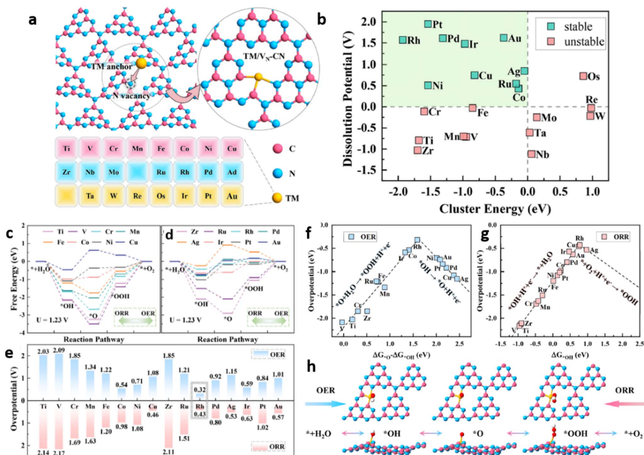
Fig. 32 (a) Schematic representation of various transition metals (TM) based SACs on VN-CN, (b) stability of TM/ \text{VN-CN} based on cluster energy ( E_{\text{Cluster}} < 0 \text{ eV} ) and dissolution potential ( U_{\text{diss}} > 0 \text{ eV} ), the free energy diagrams of TM/ \text{VN-CN} (c) from Ti to Cu and (d) from Zr to Au related to both OER and ORR at the equilibrium potential of 1.23 V, (e) The OER and ORR overpotentials of TM/ \text{VN-CN} (from Ti to Au), the volcano plots of (f) OER ( -\eta_{\text{OER}} vs. \Delta G^*\text{O} - \Delta G^*\text{OH} ) and (g) ORR ( -\eta_{\text{ORR}} vs. \Delta G^*\text{OH} ) on TM/ \text{VN-CN} , (h) OER and ORR intermediate structures adsorbed on Rh/ \text{VN-CN} . Reproduced with permission from ref. 10. Copyright 2021 American Chemical Society.
