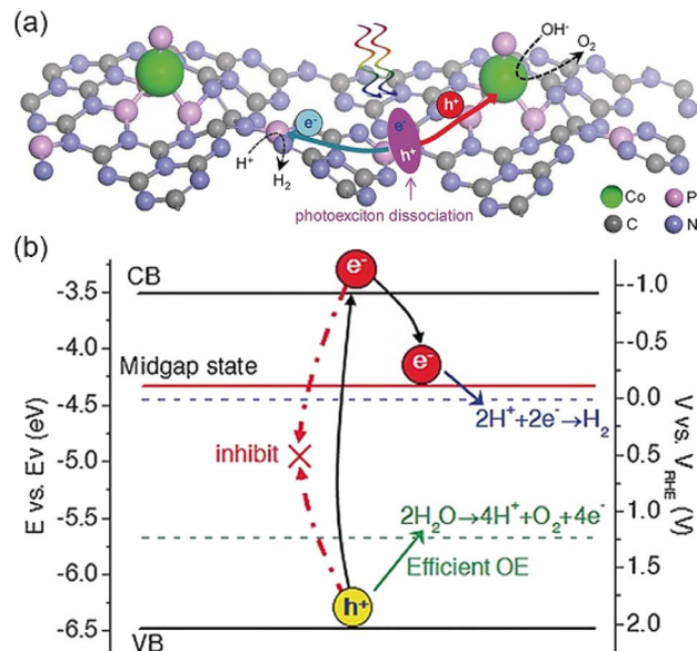
Fig. 7 (a) Schematic illustration of the solar-driven overall water splitting on the \text{Co}_1 -phosphide/PCN photocatalyst, in which the photo-generated electrons and holes ( \text{h}^+ ) are spatially separated. (b) Electronic band structure diagram for the \text{Co}_1 -phosphide/PCN photocatalyst. Copyright 2017, Wiley-VCH.
