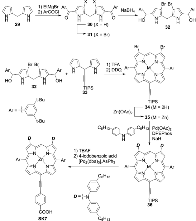
Scheme 5 Synthesis of SK7 with two donor moieties at β-positions. TFA = trifluoroacetic acid; DPEPhos = bis[(2-diphenylphosphino) phenyl]ether; [Pd 2 (dba) 3 ] = tris(dibenzylideneacetone)dipalladium(0).
