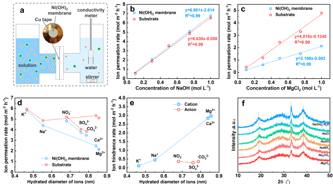
Fig. 4 (a) Schematic of \text{Ni}(\text{OH})_2 membrane test setup. Ion permeation rates under different concentrations of (b) NaOH and (c) \text{MgCl}_2 solutions. (d) Ion permeation rate versus ion hydrated diameter of the substrate and \text{Ni}(\text{OH})_2 -membrane-coated substrate. (e) The calculated ion hindrance rate for the \text{Ni}(\text{OH})_2 membrane. (f) XRD patterns of \text{Ni}(\text{OH})_2 membrane powder after immersion in different solutions.
