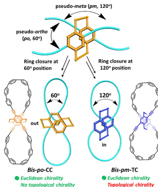
Scheme 1 Cartoon illustrations of regioselective synthesis of isomers bis-po -CC (CC = classical chirality) and bis-pm -TC (TC = topological chirality) with a differently oriented [2.2]PCP core in which the ethylene bridges are located out of and in the lemniscular framework, respectively.
