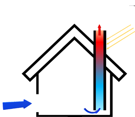
Fig. 11 Schematic of solar chimney.
