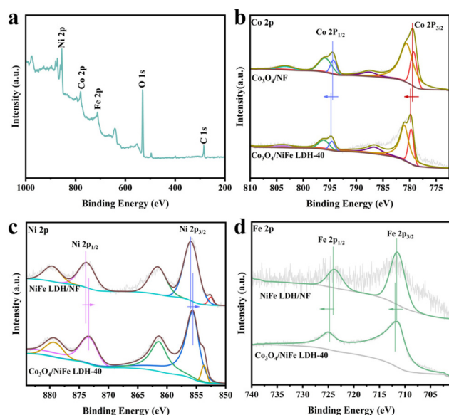
Fig. 2 (a) XPS survey spectrum of \text{Co}_3\text{O}_4/\text{NiFe LDH-40} . (b) Co 2p, (c) Ni 2p and (d) Fe 2p XPS spectra of related materials.
