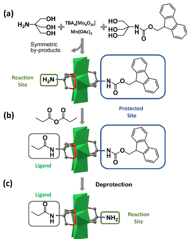
Fig. 3 (a) Synthesis method of the “universal” asymmetric Mn-Anderson precursor: \text{NH}_2-\text{MnMo}_6-\text{Fmoc} . (b) Synthesis method of \text{C}_2\text{H}_5\text{CONH}-\text{MnMo}_6-\text{Fmoc} . (c) Removal of the Fmoc group. Color code: \{\text{MoO}_6\} , green octahedron; \{\text{MnO}_6\} , red octahedron; C, gray.
