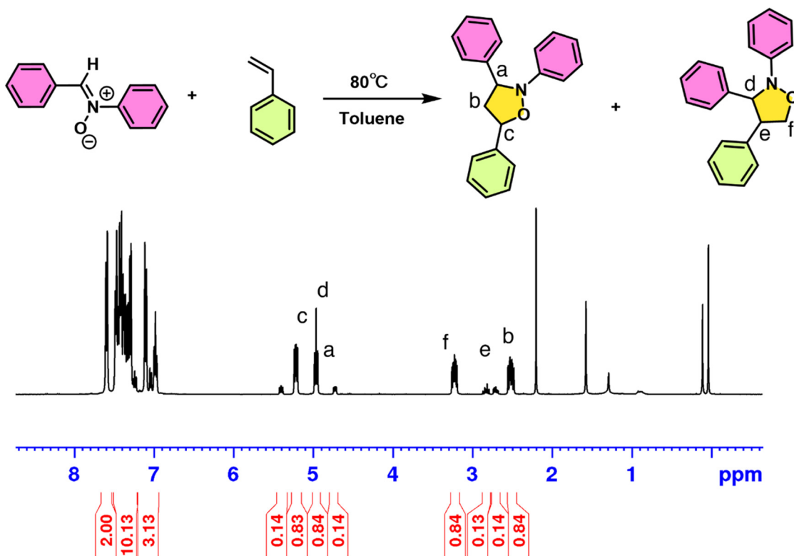
Fig. 5 ^1\text{H} NMR spectrum of the cycloadduct formed from styrene and N -1-diphenylmethanimine oxide and the peaks present at \delta = 2.5 ppm– 3.5 ppm and 4.5 ppm– 5.5 ppm confirms the formation of the cycloadduct.
