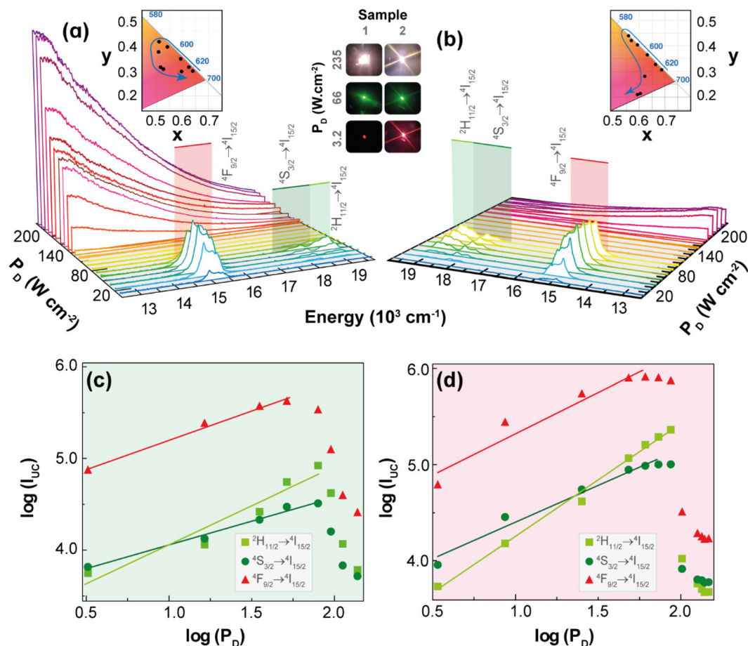
Fig. 2 Emission spectra as a function of the excitation power density, P_D , for (a) 1 and (b) 2, both samples in powders, normalized to the 4F_{9/2} \rightarrow 4I_{15/2} transition. A short pass filter (cut-off at 850 nm) was used. The insets show photographs of the samples at selected P_D values together with the CIE-1935 chromaticity diagrams with the colour coordinates for increasing P_D values between 3 and 235 \text{W cm}^{-2} . The corresponding double-log plots of the integrated intensities, I_{UC} , of selected \text{Er}^{3+} transitions as a function of P_D are presented in (c) and (d), respectively. The lines are the best fits to the data using straight lines ( r^2 > 0.99 ).
