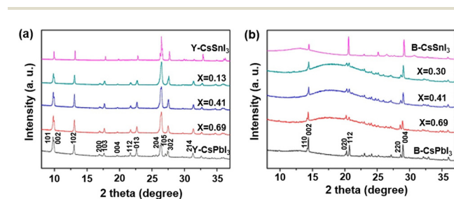
Fig. 7 XRD patterns of (a) Y-phase CsPb x Sn 1-x I 3 NWs and (b) B-γ phase CsPb x Sn 1-x I 3 NWs. Reproduced from ref. 78 with permission from the American Chemical Society. Copyright 2018.
